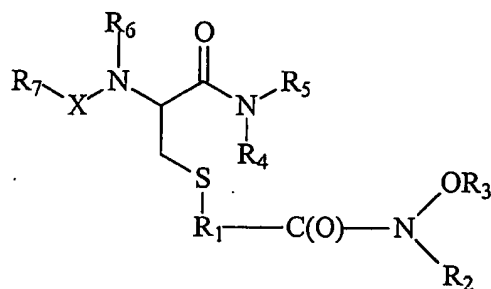
(IIIa)
